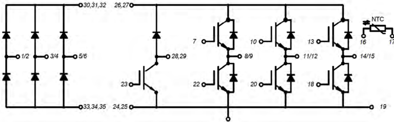
Figure 17. Circuit Diagram
