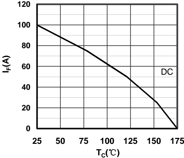
Figure 16. Forward current vs Case temperature Diode -inverter
