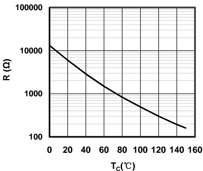
Figure 14. NTC Characteristics
