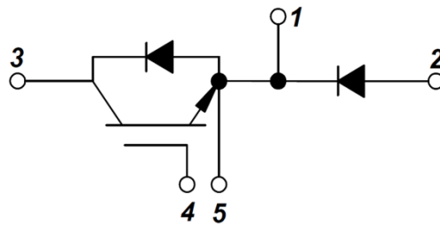
Figure 13. Circuit Diagram
