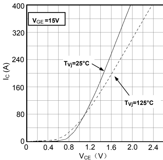
Figure1. Typical Output characteristics IGBT-inverter
