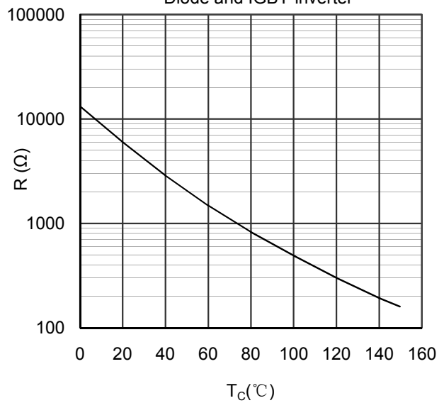
Figure 13. NTC Characteristics
