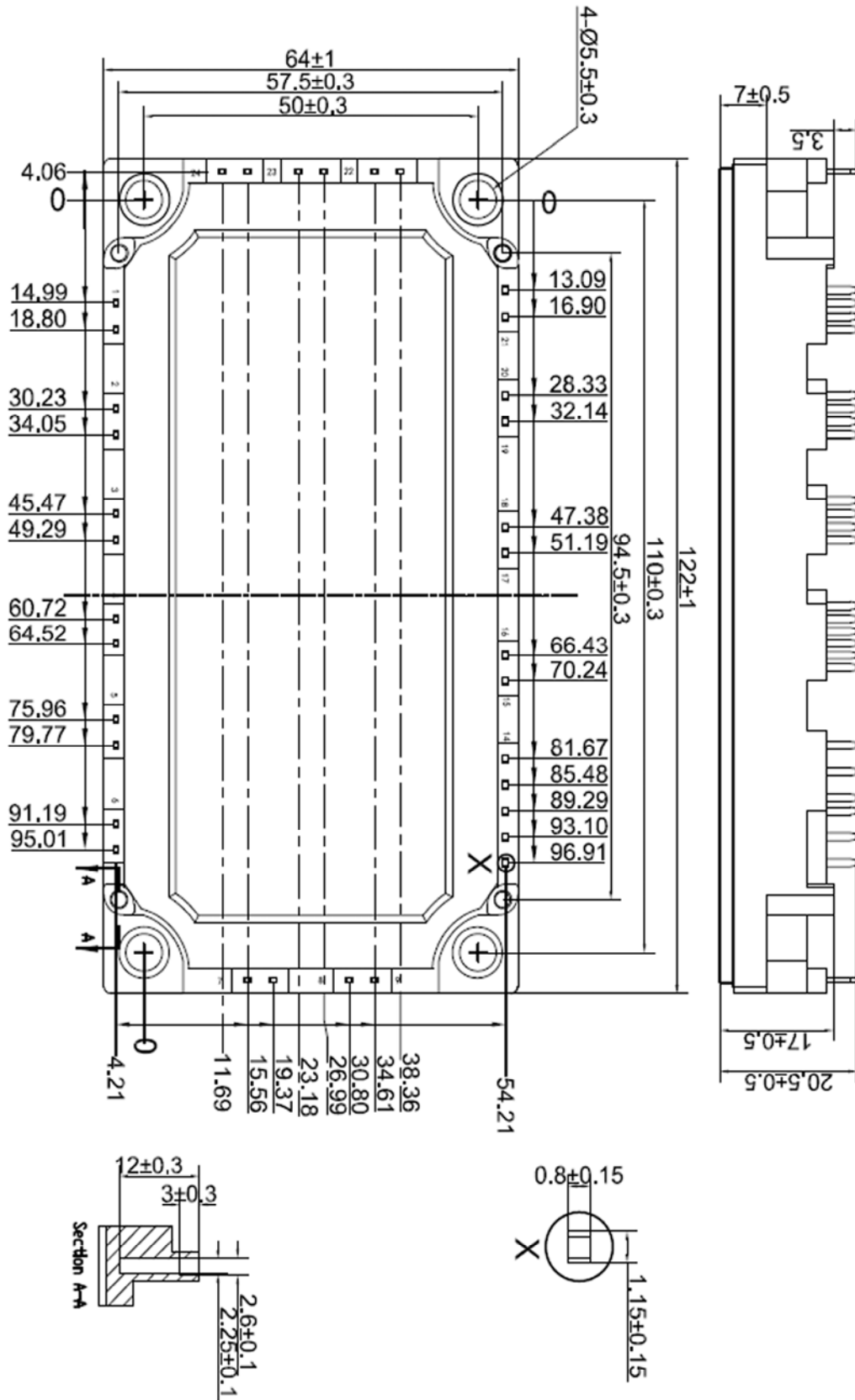
Dimensions in (mm) Figure 18. Package Outline
