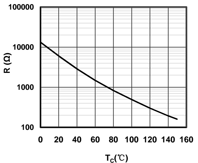
Figure 14. NTC Characteristics
