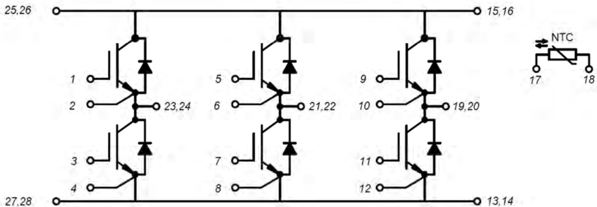
Figure 14. Circuit Diagram
