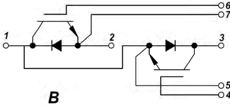
Figure 13. Circuit Diagram
