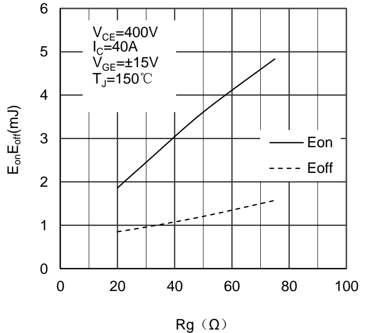
Figure 4. Switching Energy vs Gate Resistor IGBT
