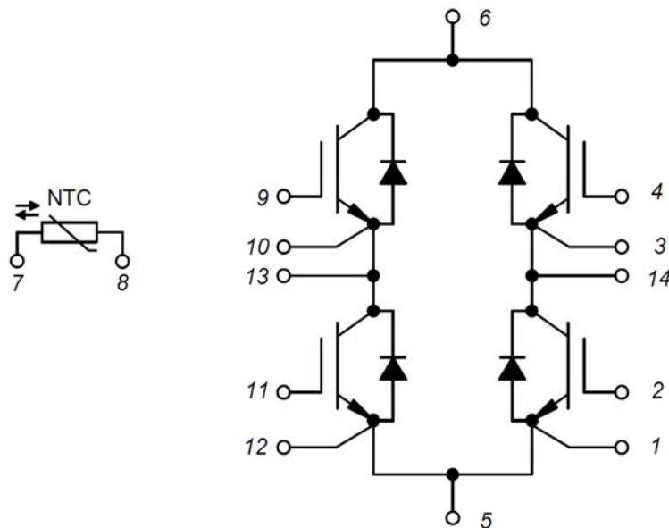
Figure 14. Circuit Diagram
