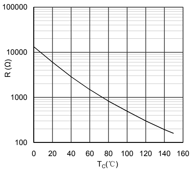
Figure 14. NTC Characteristics
