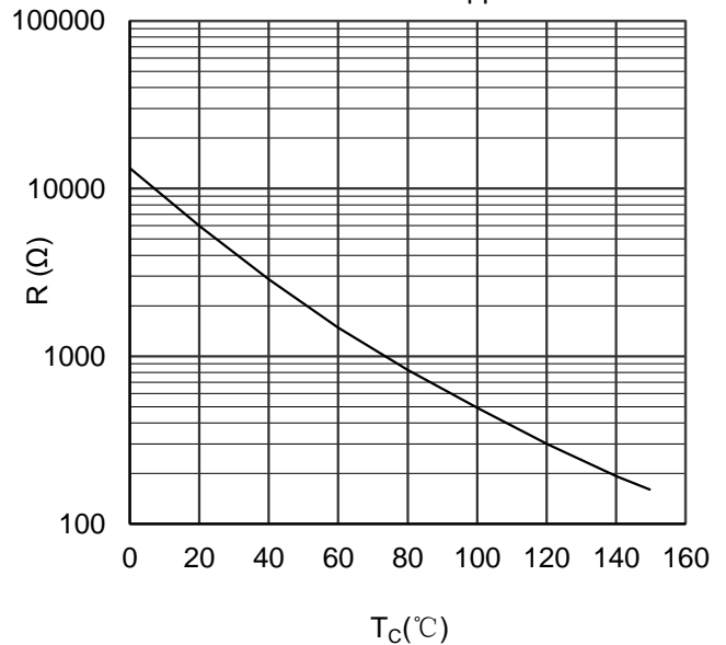
Figure 14. NTC Characteristics
