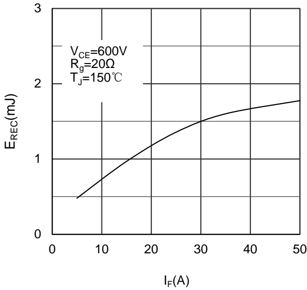
Figure 9. Switching Energy vs Forward Current Diode-inverter
