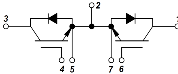
Figure 13. Circuit Diagram
