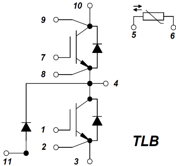
Figure 14. Circuit Diagram
