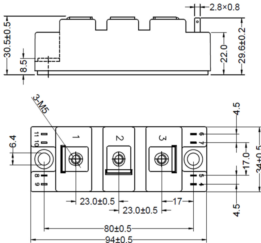
Figure 14. Package Outline
