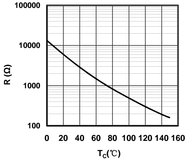
Figure 13. NTC Characteristics
