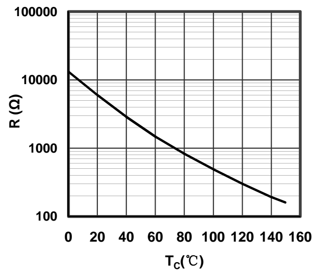
Figure 14. NTC Characteristics
